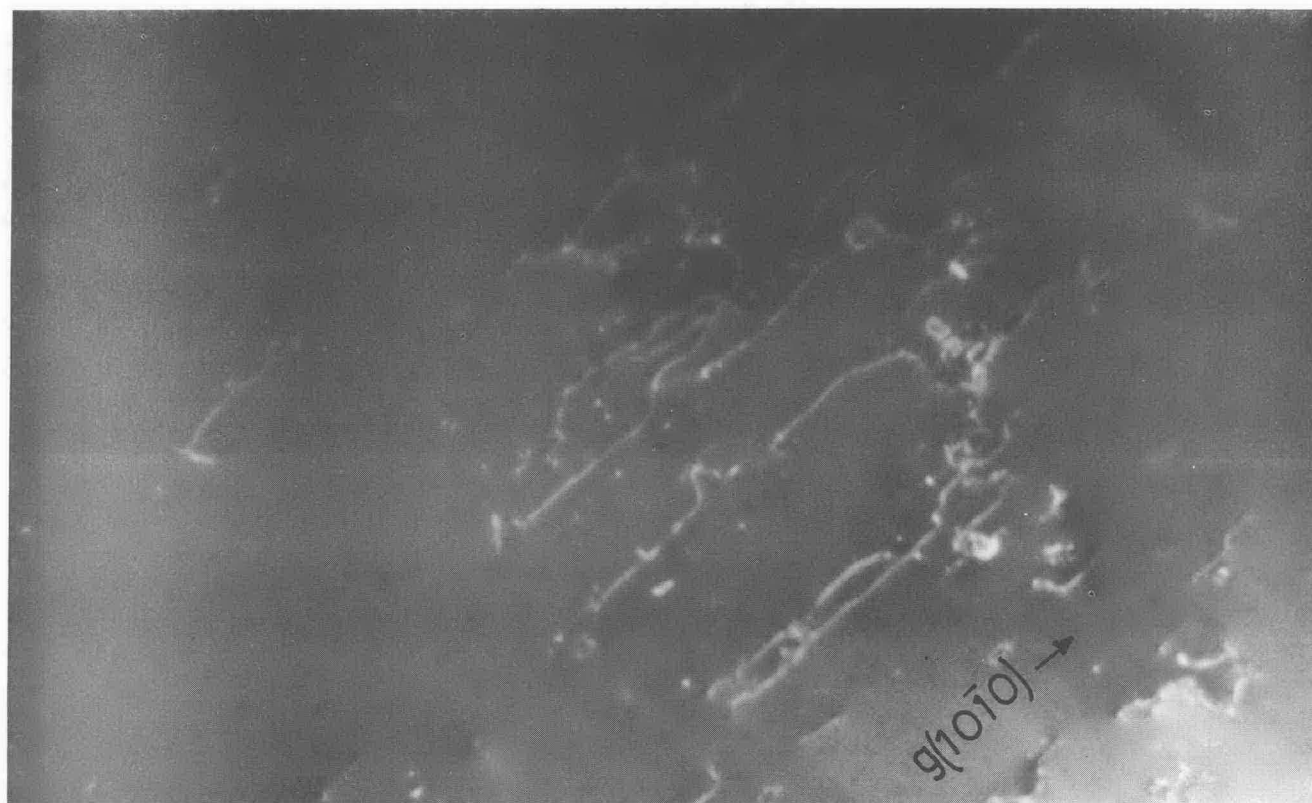
Fig. 9 - Electron Transmission Micrographs of Crystal ISR-11 Foil Cut Parallel to (11\bar{2}0) Showing Contrast Effects for (a) g(0002) and (b) g(10\bar{1}0) . Mag. 37,500X
